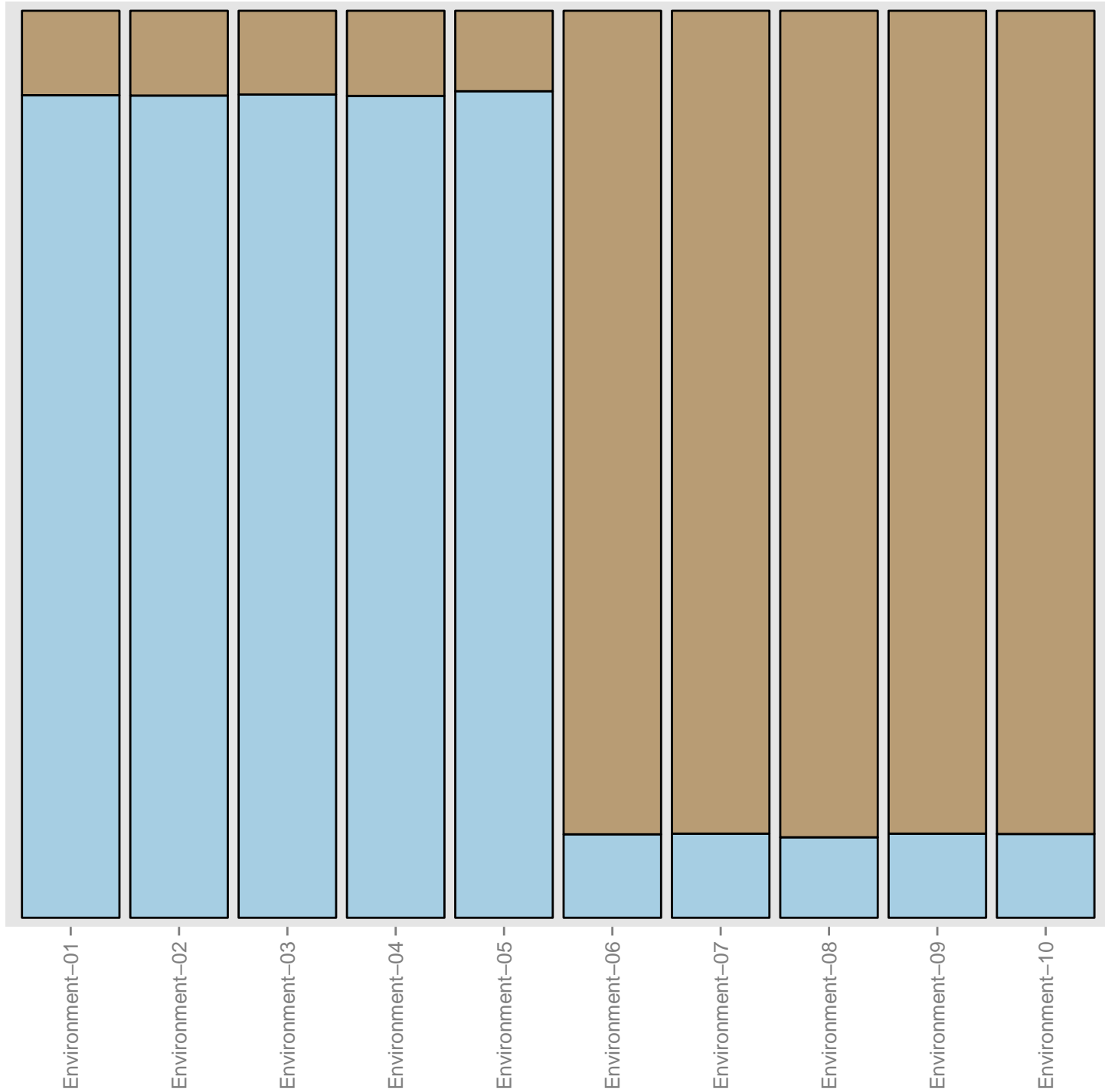
Distribution of Oligotypes Among Samples for mock-env-aligned
